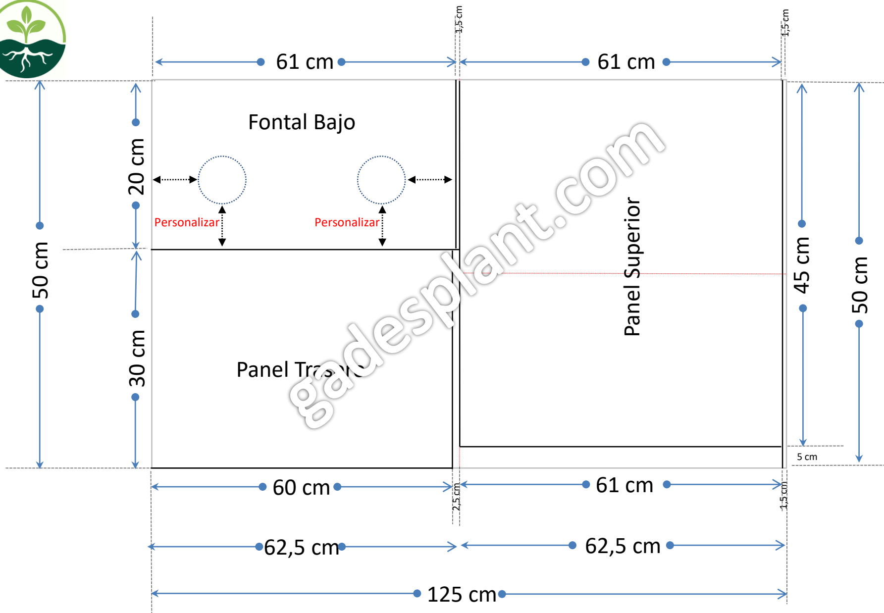
Corte Panel Poliestireno PS6 – 50X125 / 4MM
